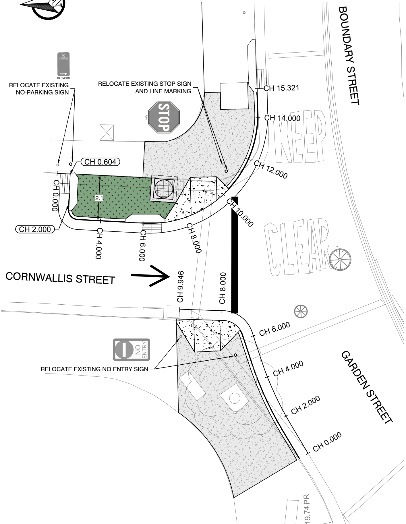
KERB EXTENSION, CORNWALLIS STREET, REDFERN NOT TO SCALE
